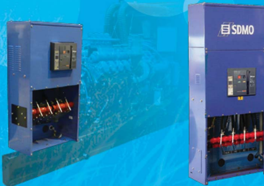
2 connection unit with air cooler unit (with integrated air cooler unit on the lower section if necessary)
